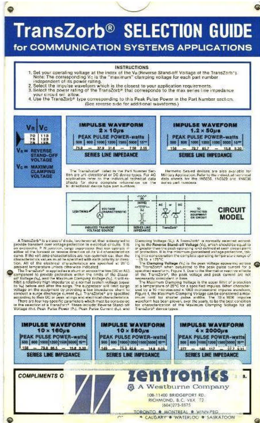
Figure 1. TransZorb Selection Guide
