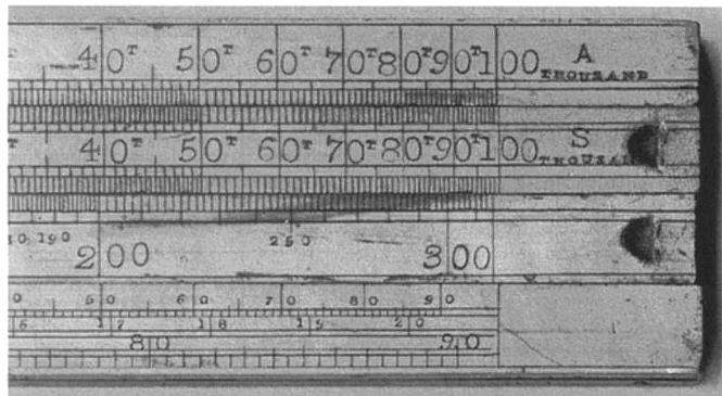
Figure 3. This rule by Hoare is about 32.3 inches long. There are six full cycles on the A and S scales. At the left end, they start at 0.1, while at the right end (shown) they end at 100,000.
